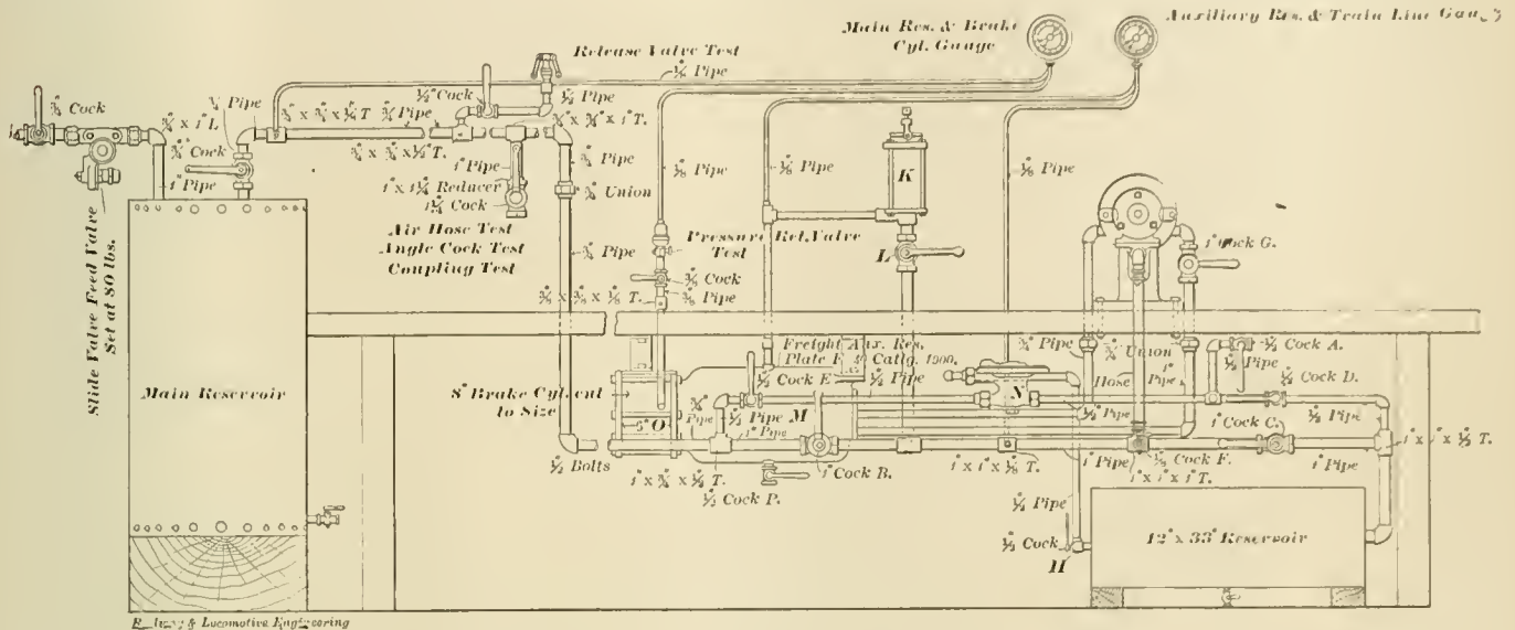
SHOP TEST RACK FOR REPAIRED TRIPLES—SIDE VIEW.
